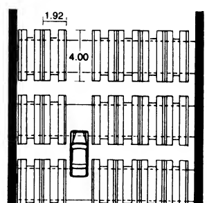
⑩ Pallets moving along rows (Klaus system)
